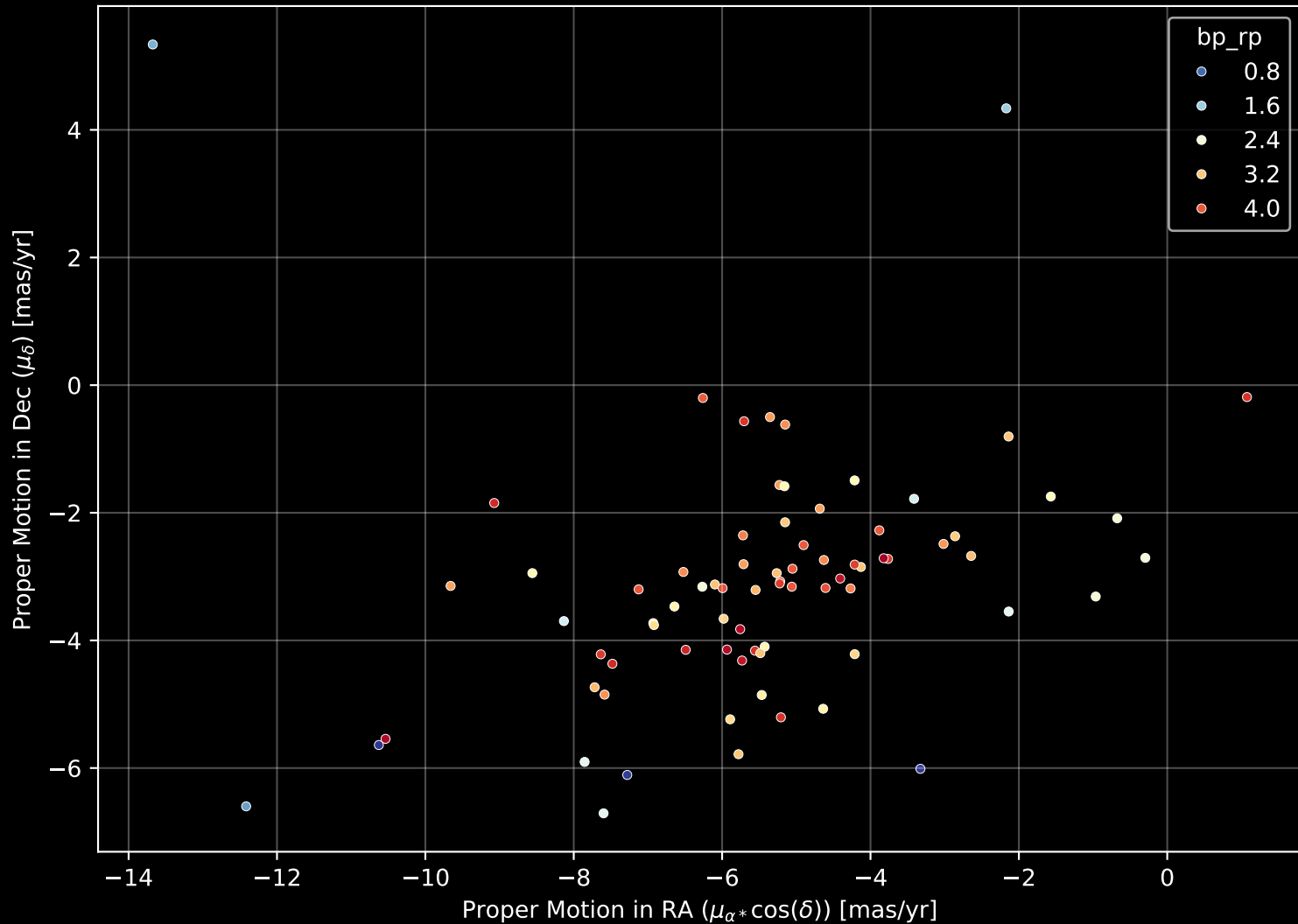
APOGEE DR17 Field: [317+00] Proper Motion Diagram (n= 77)
