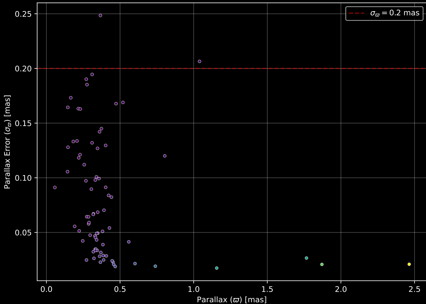
APOGEE DR17 Field: [317+00] Parallax Quality (n= 77)
