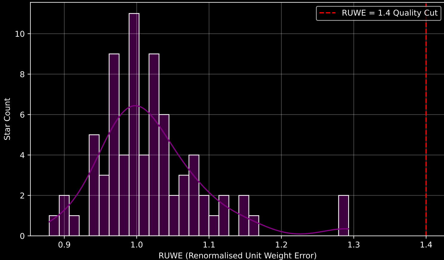
GAPOGEE DR17 Field [317+00] RUWE Distribution (n= 74)
