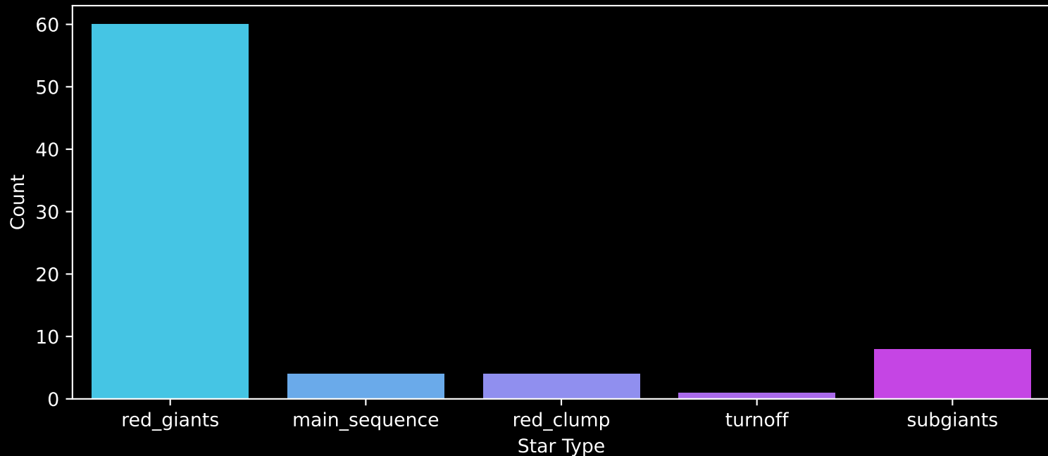
APOGEE DR17 Field: [317+00] Count plot of Star Type
