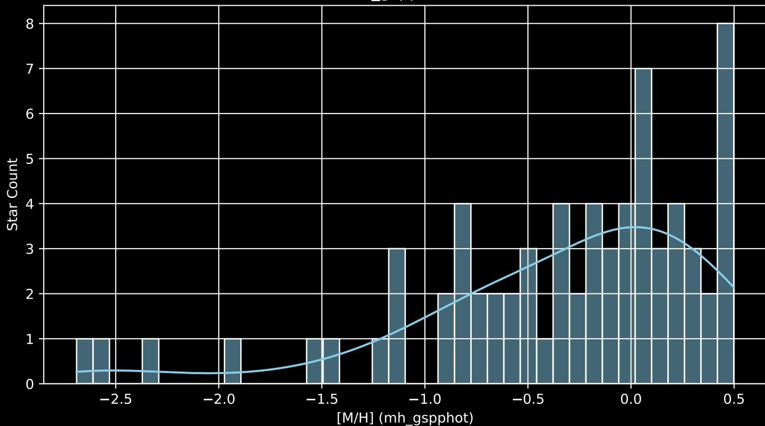
APOGEE DR17 Field: [317+00 [M/H] (mh_gspphot) (n= 70)
